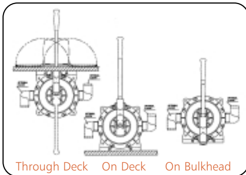
On Bulkhead
